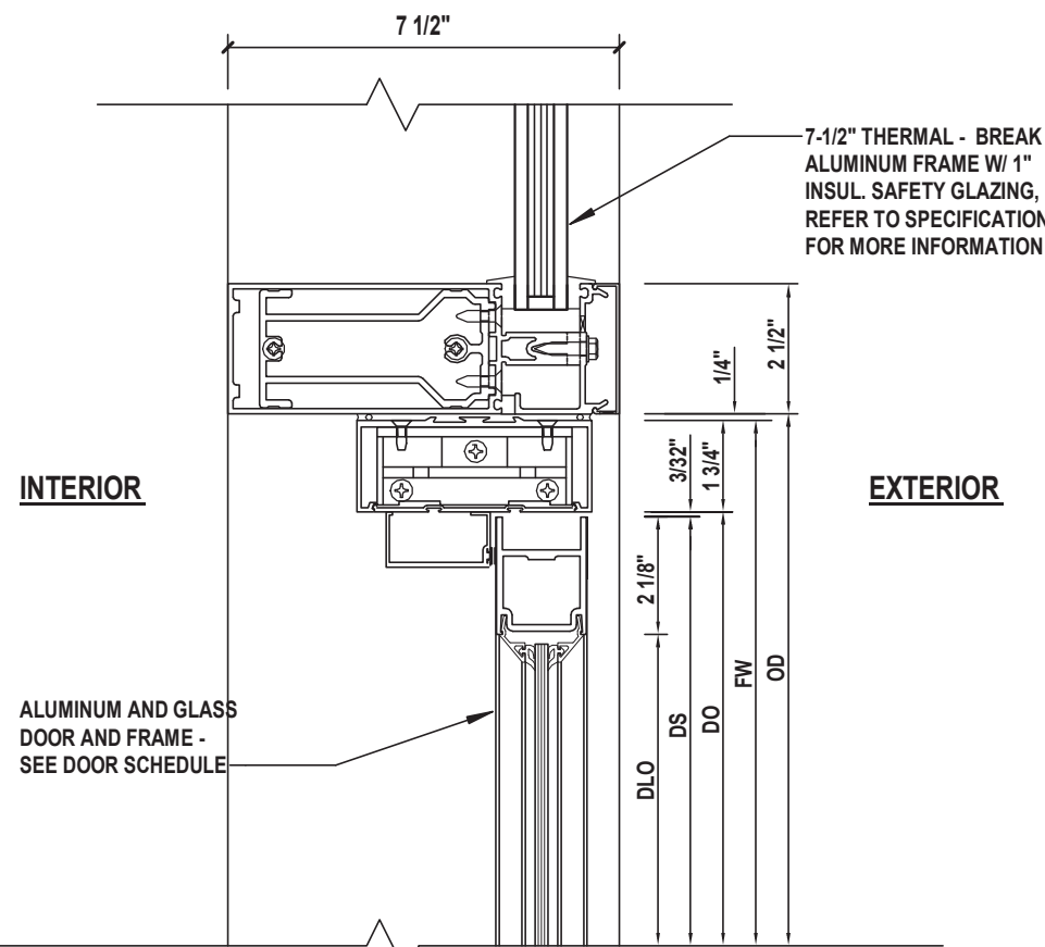
2 Door Head Detail SCALE: 3/4" = 1'-0"
