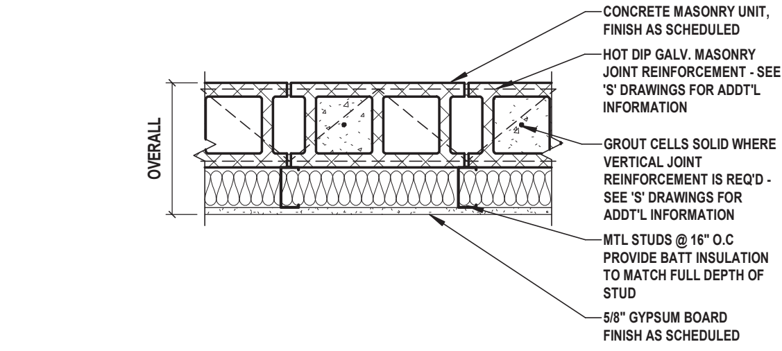
2 CMU w/ Aluminum Siding Exterior Partition
