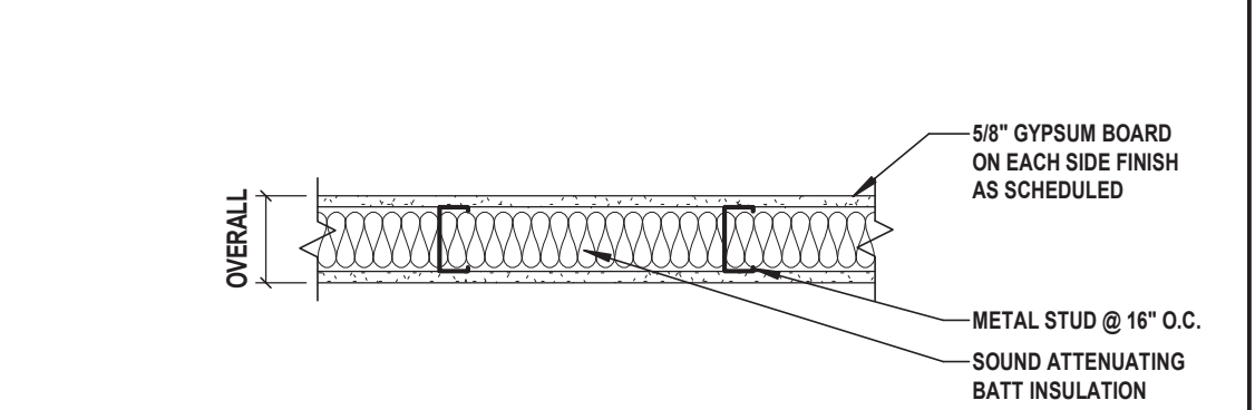
4 Metal Stud w/ Fiber Cement Panels Exterior Partition
