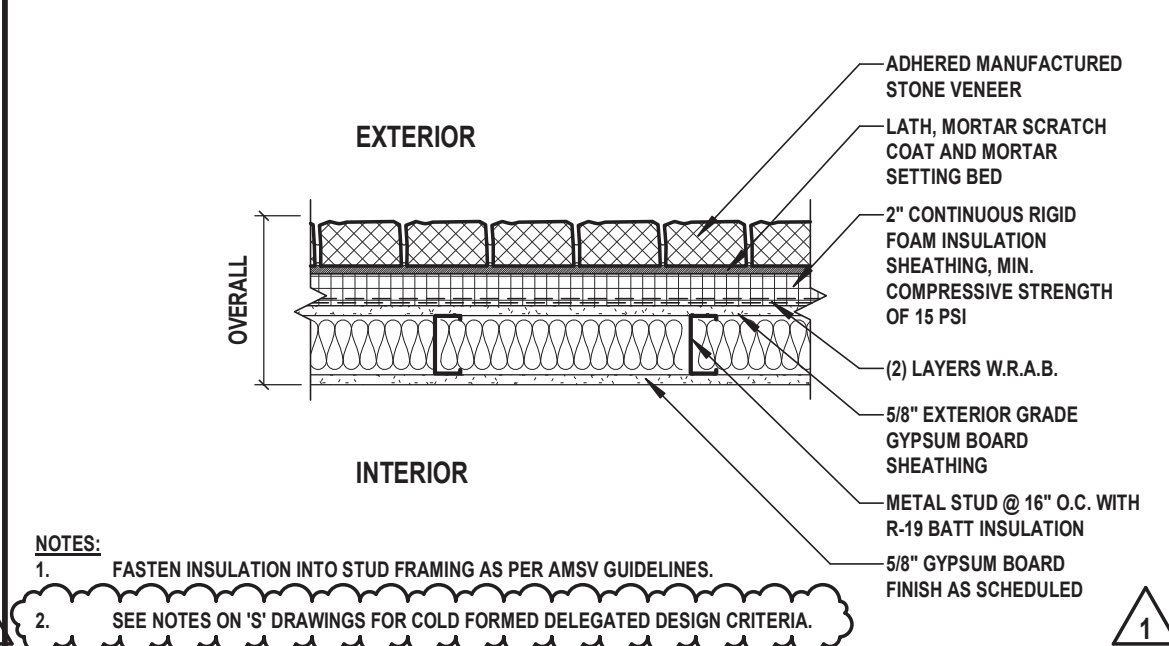
1 Masonry Veneer Exterior Partition
