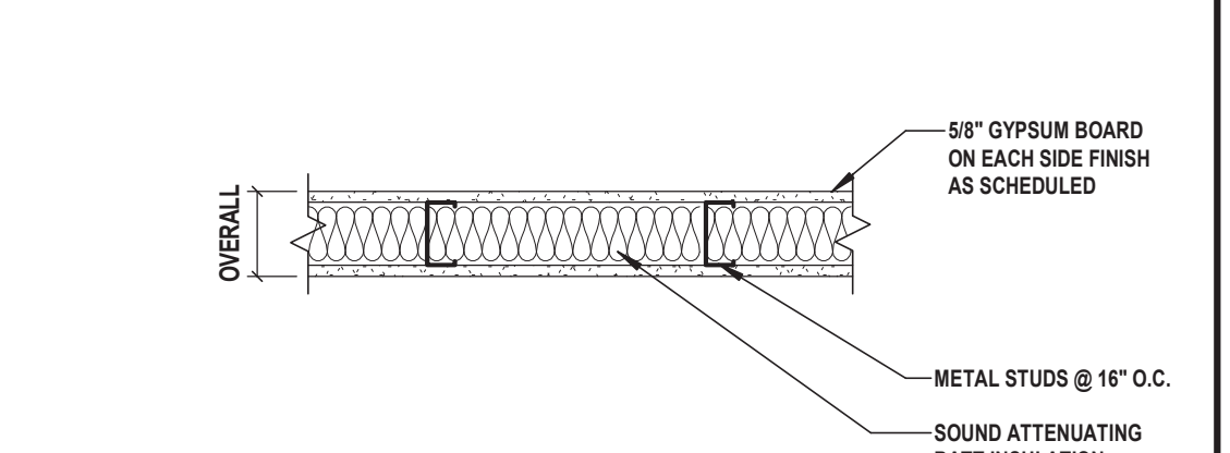
5 Metal Stud w/ Aluminum Siding Exterior Partition
