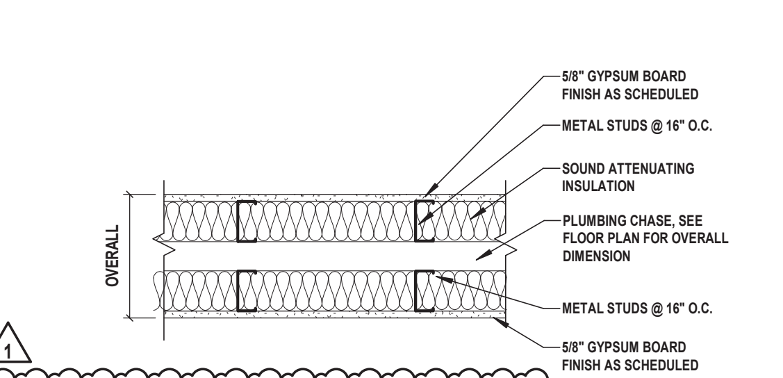
7 CMU w/ Metal Stud Interior Partition
